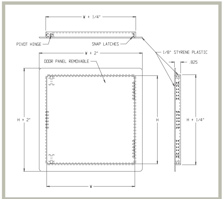
PA-3000 View of door back
